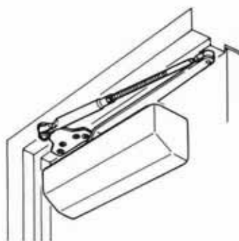
CLOSER MOUNTED ON PUSH SIDE OF DOOR
