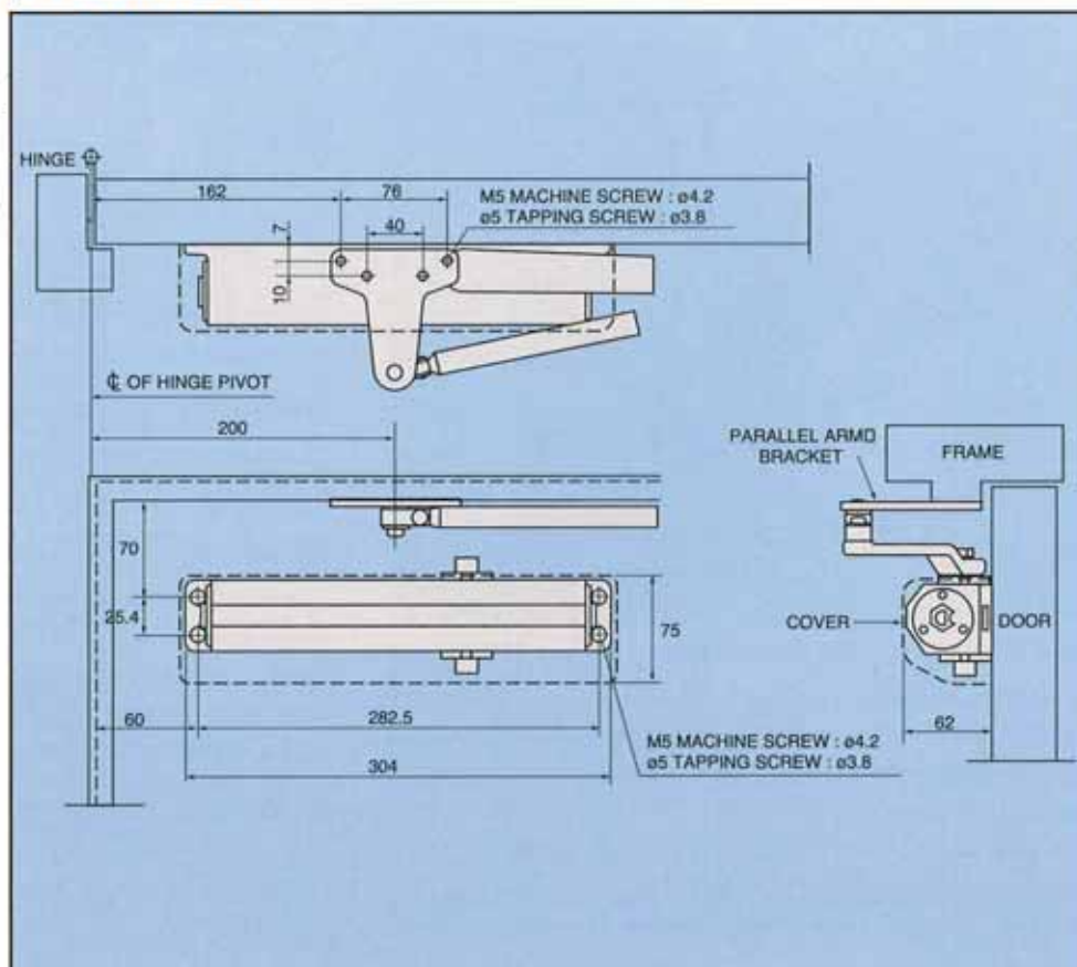
CLOSER MOUNTED ON PUSH SIDE OF DOOR
